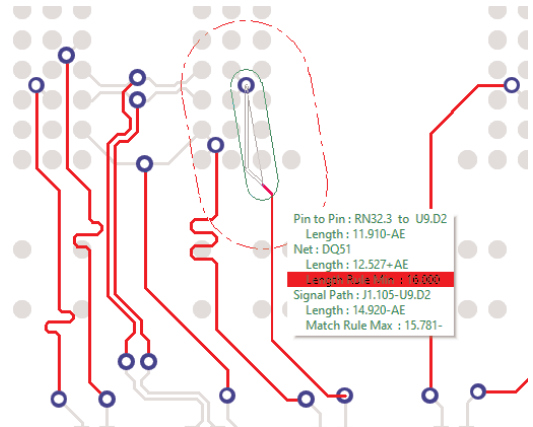
A 'head-up' display shows you colour-coded rules as the design is edited and the track lengths change
