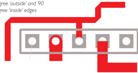
Square-ended tracks provide precise track ends when an 'open-ended' square end is required
